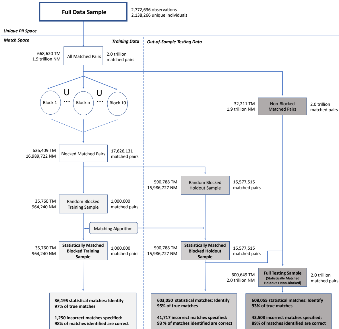
Figure 2: Model Training and Testing Overview
